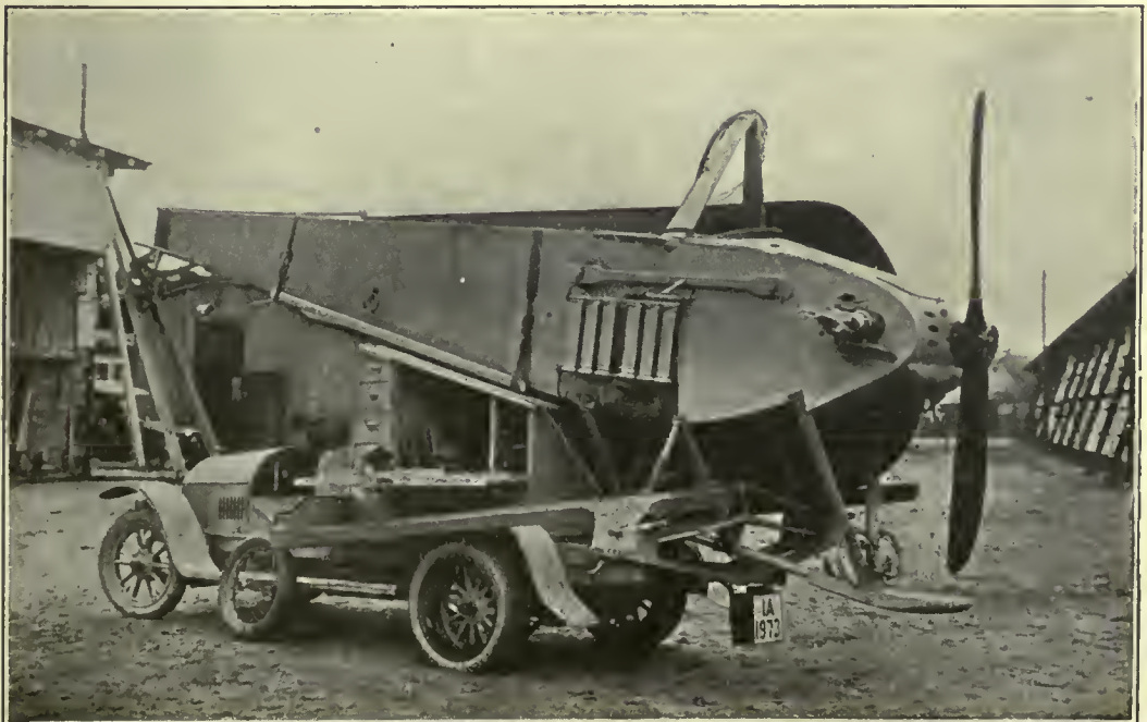
GERMAN MILITARY AEROPLANE PACKED FOR TRANSPORT ON A MOTOR.
