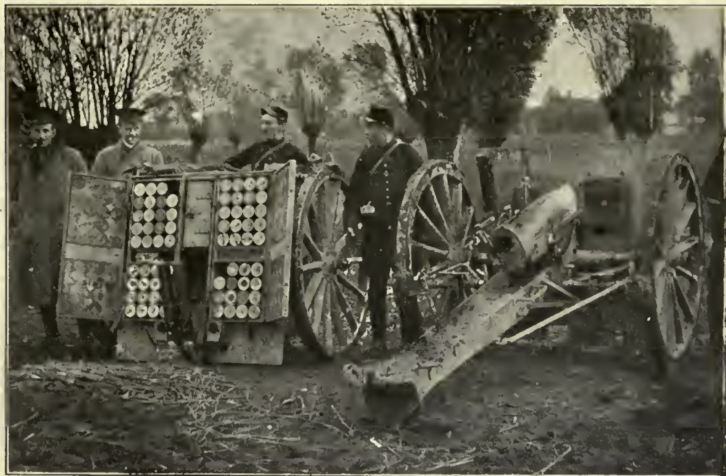
A FRENCH 75-MM. GUN, SHOWING BREECH MECHANISM AND AMMUNITION LIMBER.
