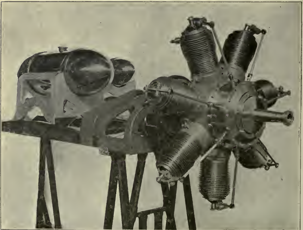
LATEST TYPE GNOME ENGINE.
